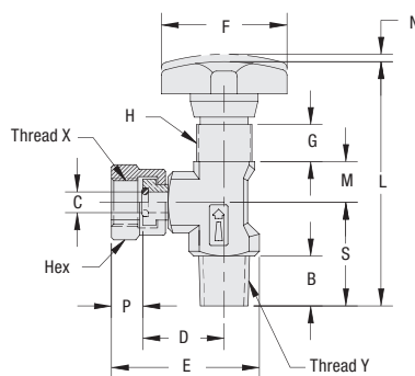
90° Version
