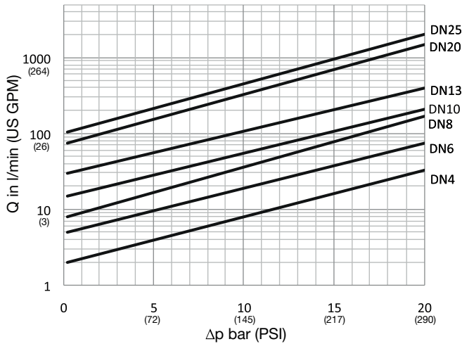
CBVL / CBVT
